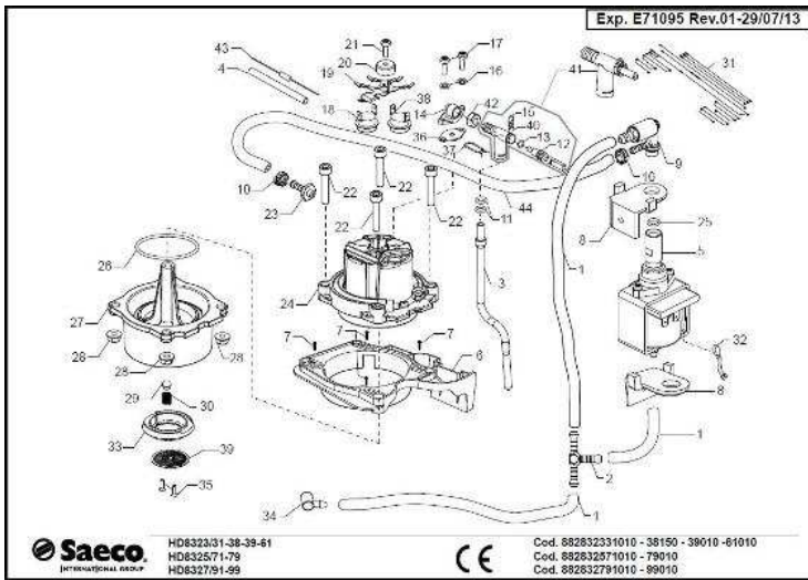
Image 4 -Aluminum Boiler
