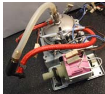
Remove the pump from the supports
