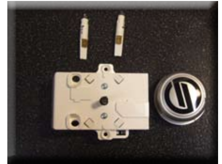
Loosen the screws as shown to remove the rotating switch
