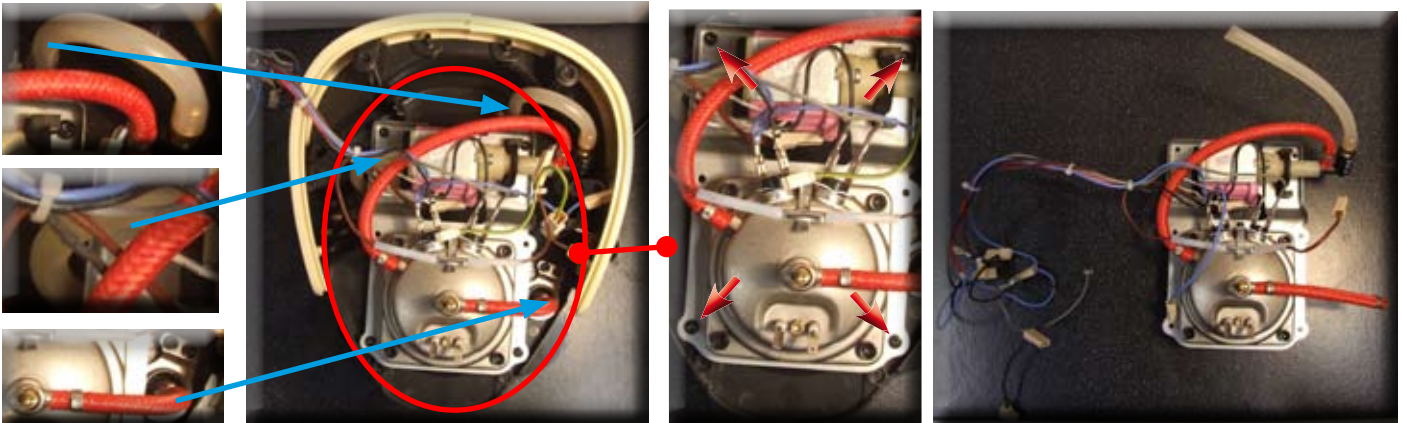
Remove the water connections and loosen the screws as shown
