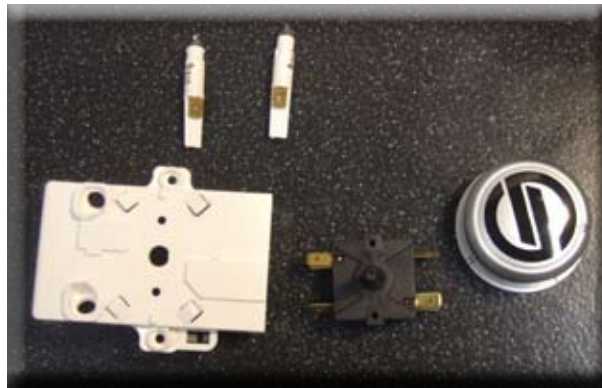
Remove the electrical connections and the two bright indicators
