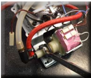
Loosen the overpressure valve
