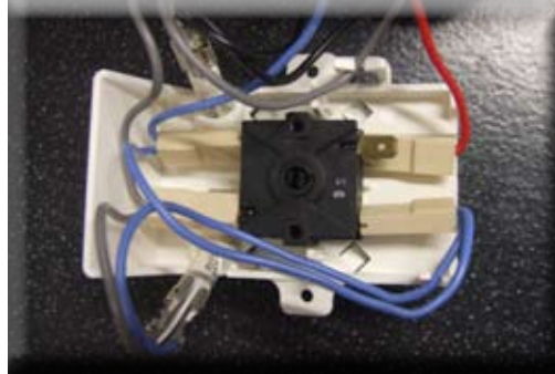
Remove the electrical connections and the two bright indicators
