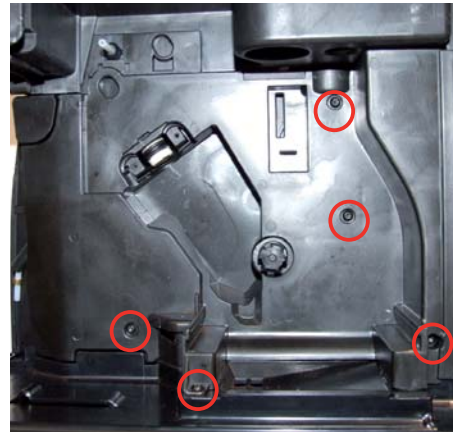
Loosen the screws as illustrated and remove the gear motor cover.
