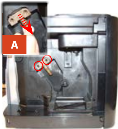
Loosen the screws as illustrated and remove the boiler pin (A).
