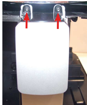
Unscrew the screws as illustrated and remove the front panel to access the screws which fix the dispenser cover into place.
