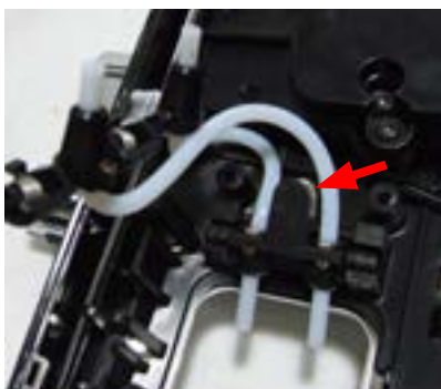
When re-mounting it, make sure to reposition the spring correctly
