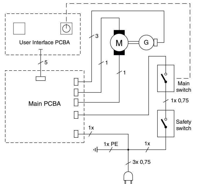
Device interconnection diagram
